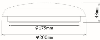
OYSDIM001-LINE DRAWINGS
