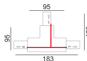
TRK1BLCON4R1 TRK1WHCON4R1
