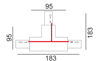
TRK1BLCON4R2 TRK1WHCON4R2
