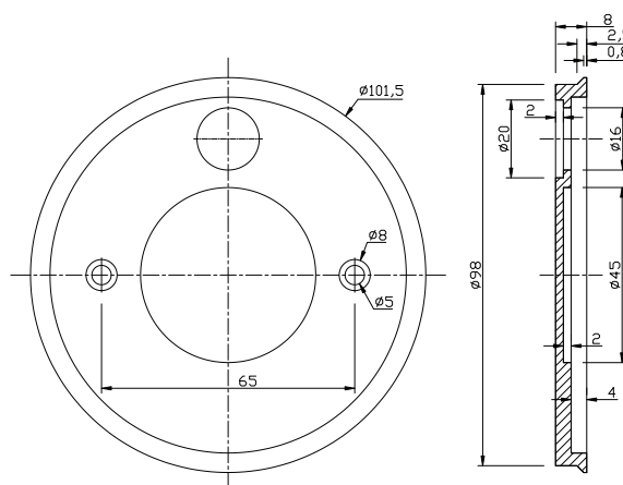
Back plate dimensions
