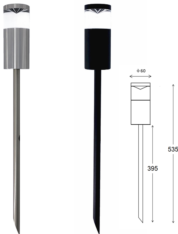
PHARE06M (Titanium Anodized Aluminium) PHARE07M (Powder Coated Black Aluminium)
