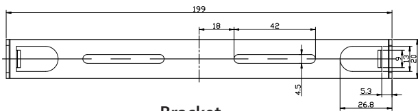
Bracket
